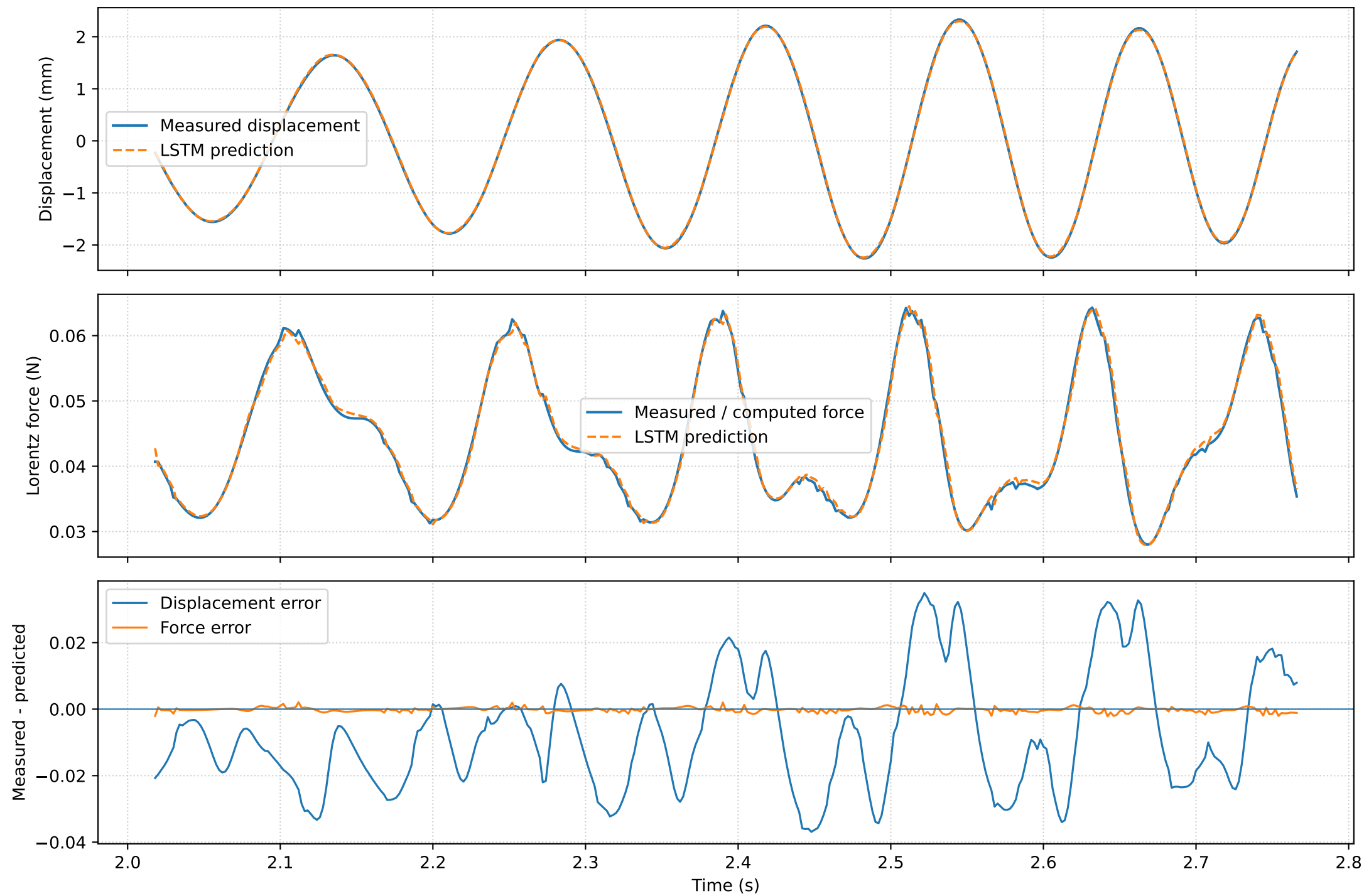
Zoomed LSTM tracking: Chirp_2 | center = 2.392 s | window = 0.750 s
